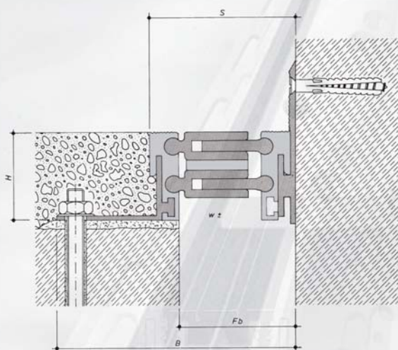
Floor to wall options, wall fixing plate may rotated 180°
